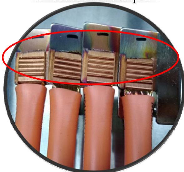
Ultrasound Welding
