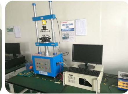
Insertion and Extraction Force Tester
